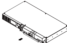
5. Replace the new battery pack. Assemble the screws, cover, cable and front panel in the reverse sequence of above steps. Recharge the unit for 4-8 hours to ensure the UPS performs expected runtime.
