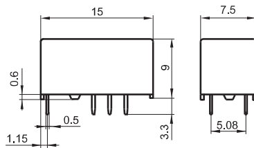
Single side stable & 1 coil latching
