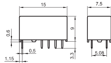
2 coils latching
