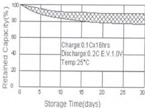
Storage Characteristics
