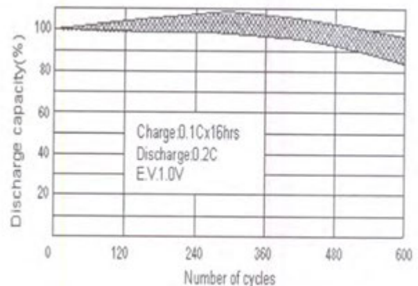
Cycle Life
