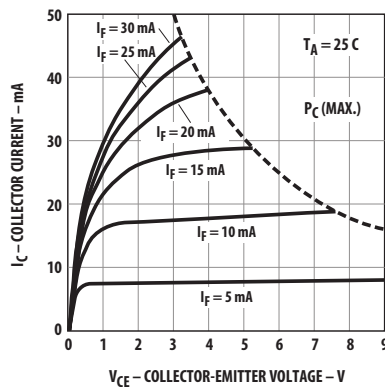
Figure 6. Collector current vs. collector-emitter voltage.
