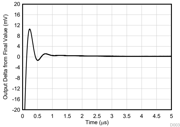
Figure 7-31. Large-Signal Step Response (Rising)
