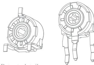
Detents details
