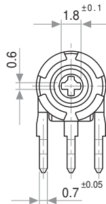
W = Adjustable from terminal side
