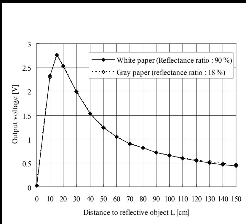
Fig. 2 Example of distance measuring characteristics (output)
