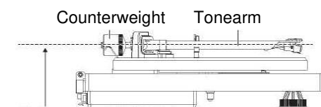
Adjust for balanced tonearm
