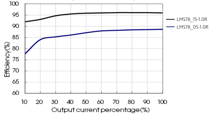
Positive output Efficiency Vs output load (Vin=Vin-nominal)
