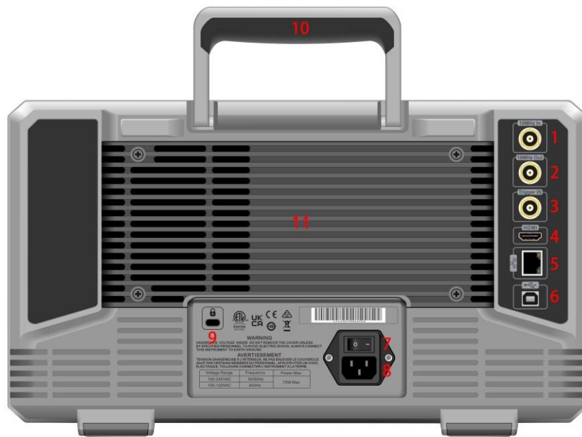
Figure 1-3 Rear Panel
