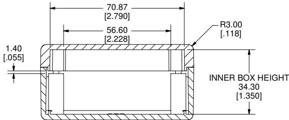
SECTION C-C SCALE 1 : 1
