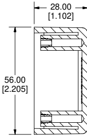
SECTION B-B SCALE 1 : 1
