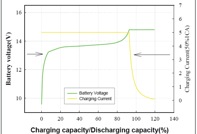
Constant voltage charging characteristic (0.5CA, 25 Celsius scale)
