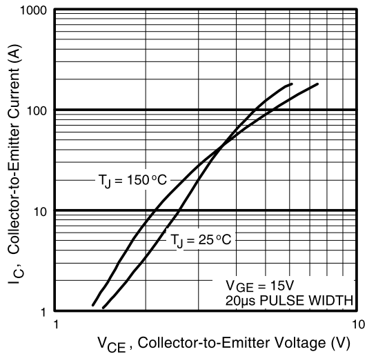
Fig. 2 - Typical Output Characteristics www.irf.com
