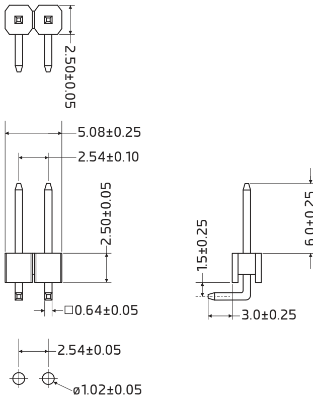
Recommended PCB Board Hole Layout
