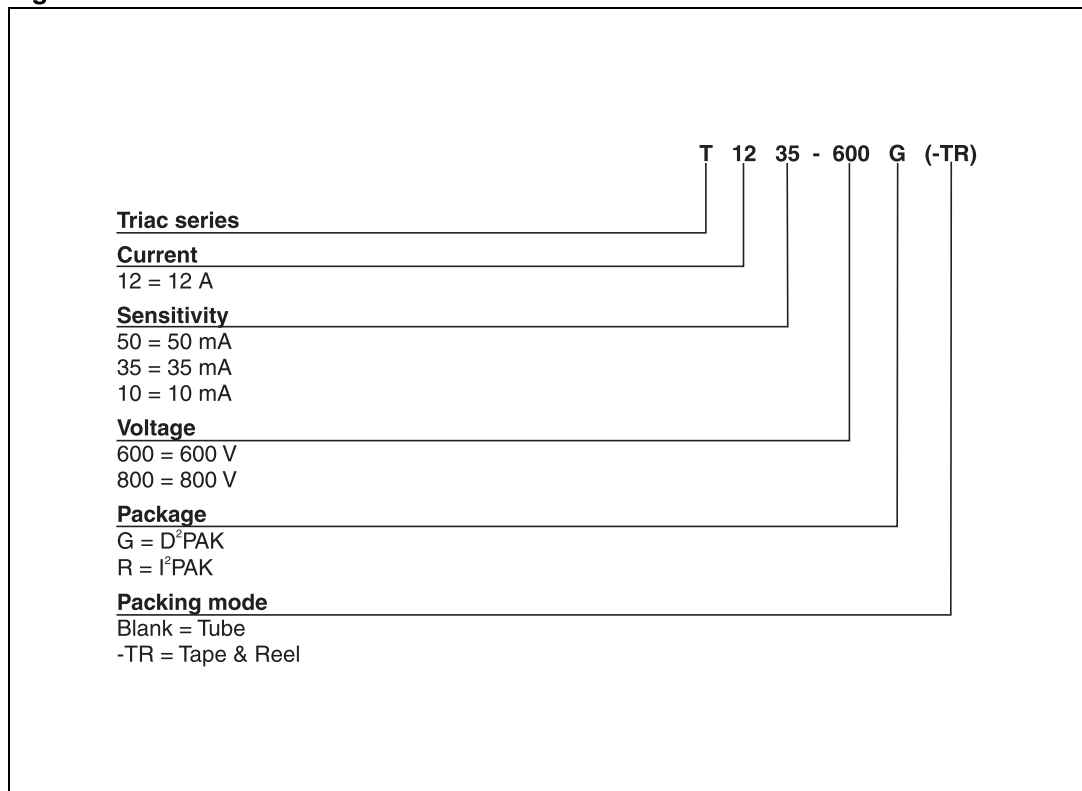
Figure 14. T12xx series
