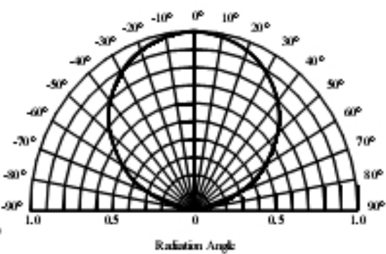
Radiation diagram
