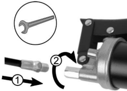
Figure 2 : Raccorder le tuyau
