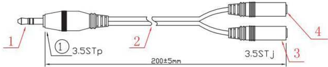
WIRING DIAGRAM
