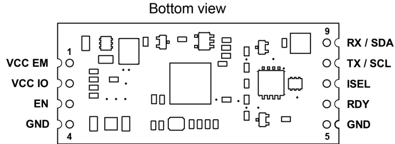
Fig. 6 Pin assignment
