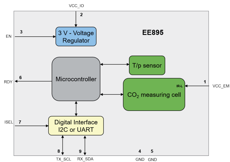
Fig. 5 Block diagram
