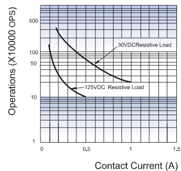
ENDURANCE CURVE
