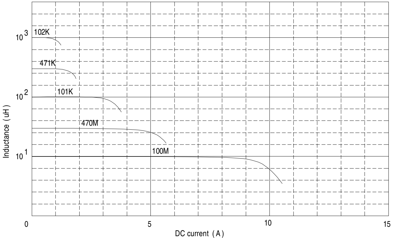
@ Inductance VS. DC superposition characteristics
