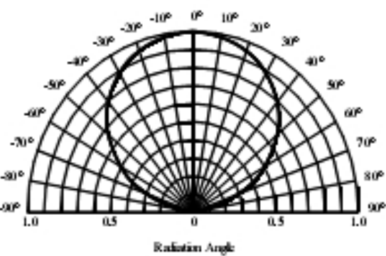
Radiation diagram
