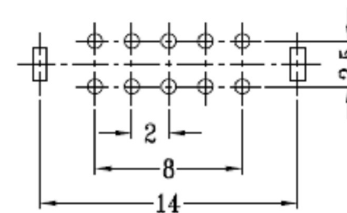
P.C.B LAYOUT BOTTOM VIEW
