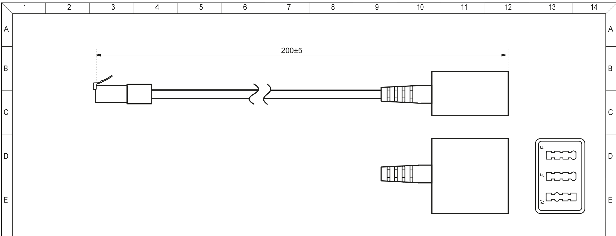
RJ45/8P4C
