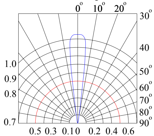
Radiation Diagram
