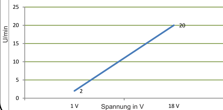
G1000-12V
