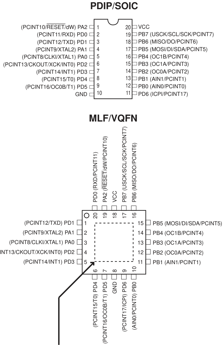
Figure 1-1. Pinout ATtiny2313A/4313
